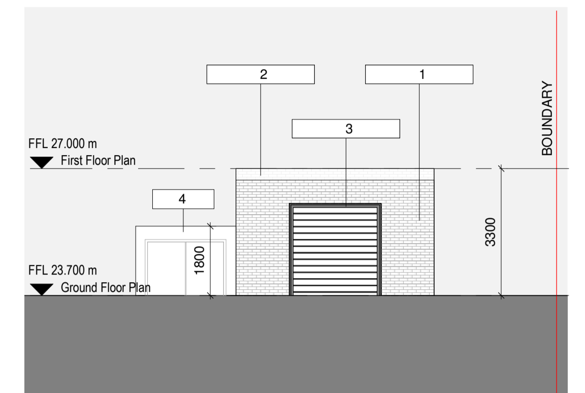
5 South Elevation 1 : 100
