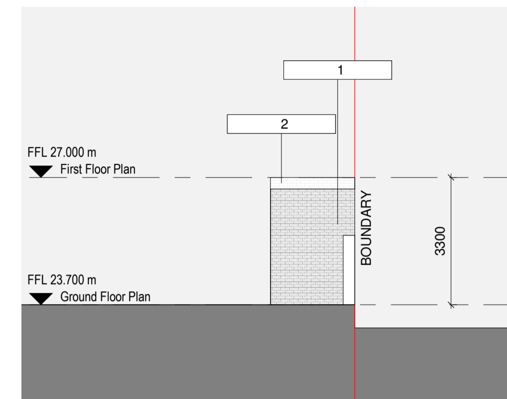
4 East Elevation 1 : 100
