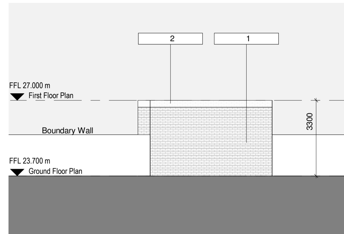
3 North Elevation 1 : 100
