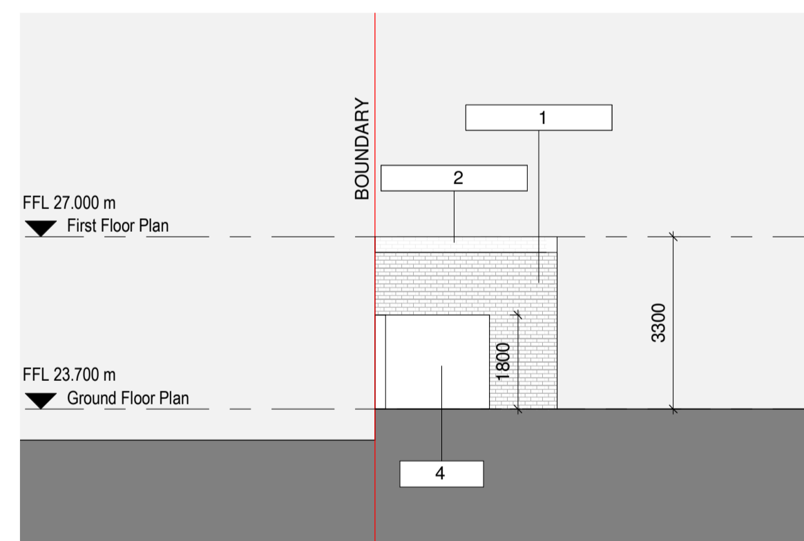
6 West Elevation 1 : 100
