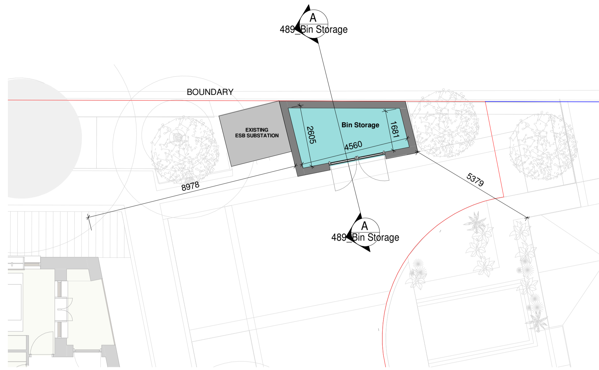
1 Ground Floor Plan_Bin Storage 1 : 100 WITH EXISTING ESB SUBSTATION
