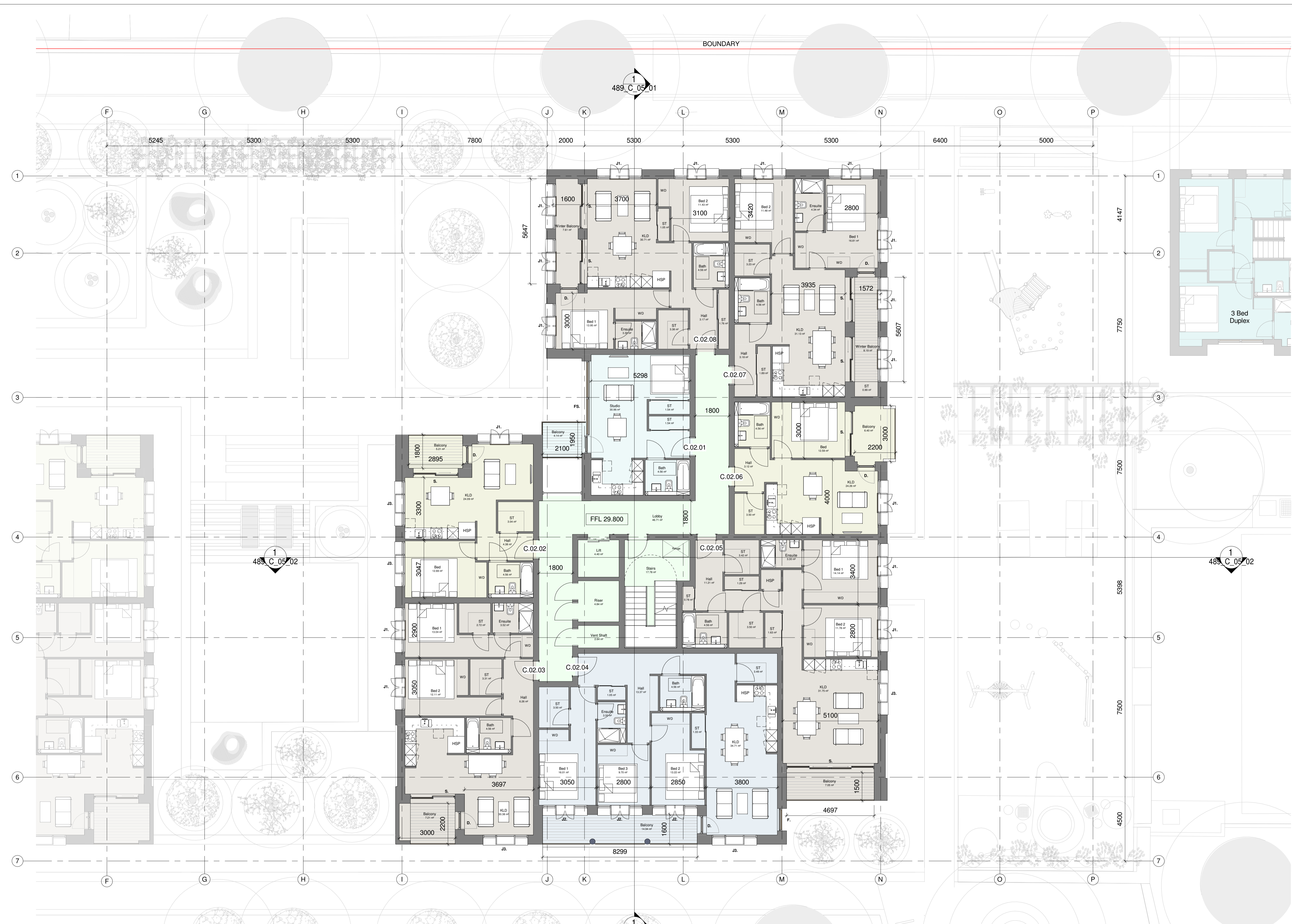
1 Second Floor Plan_Block C 1 : 100
