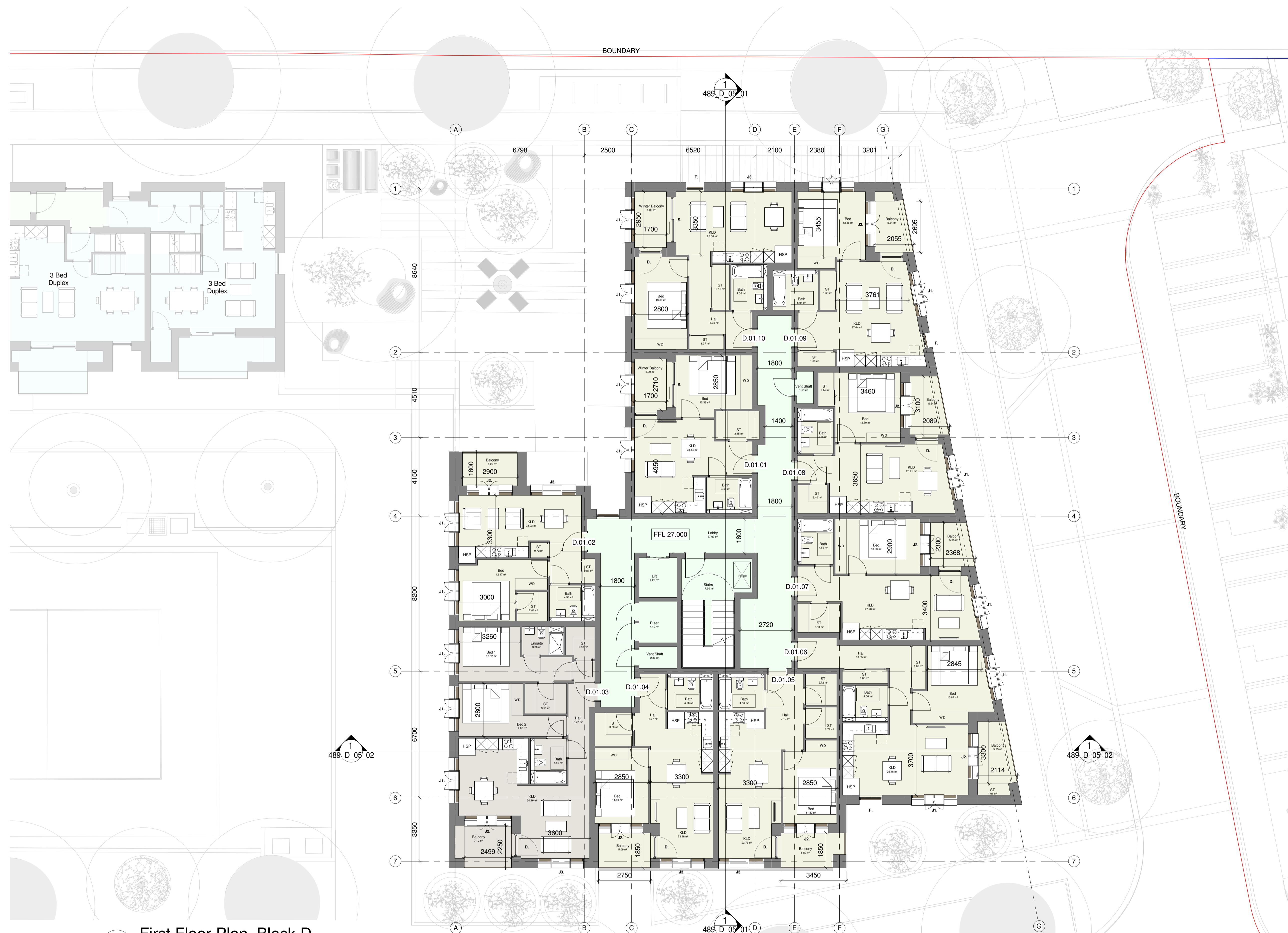
1 First Floor Plan_Block D 1 : 100
