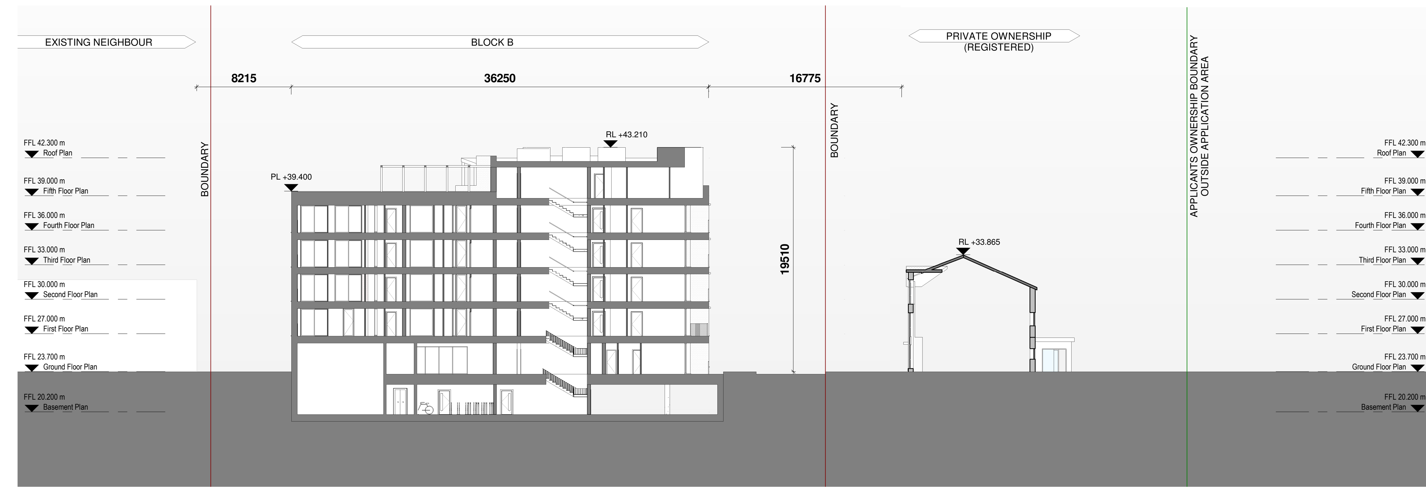
C Contextual Site Section CC 1 : 200
